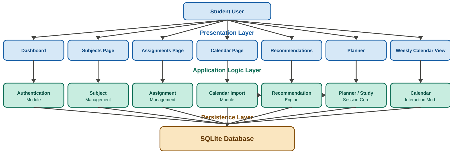
Figure 1. Building Block View of StudyFlow
