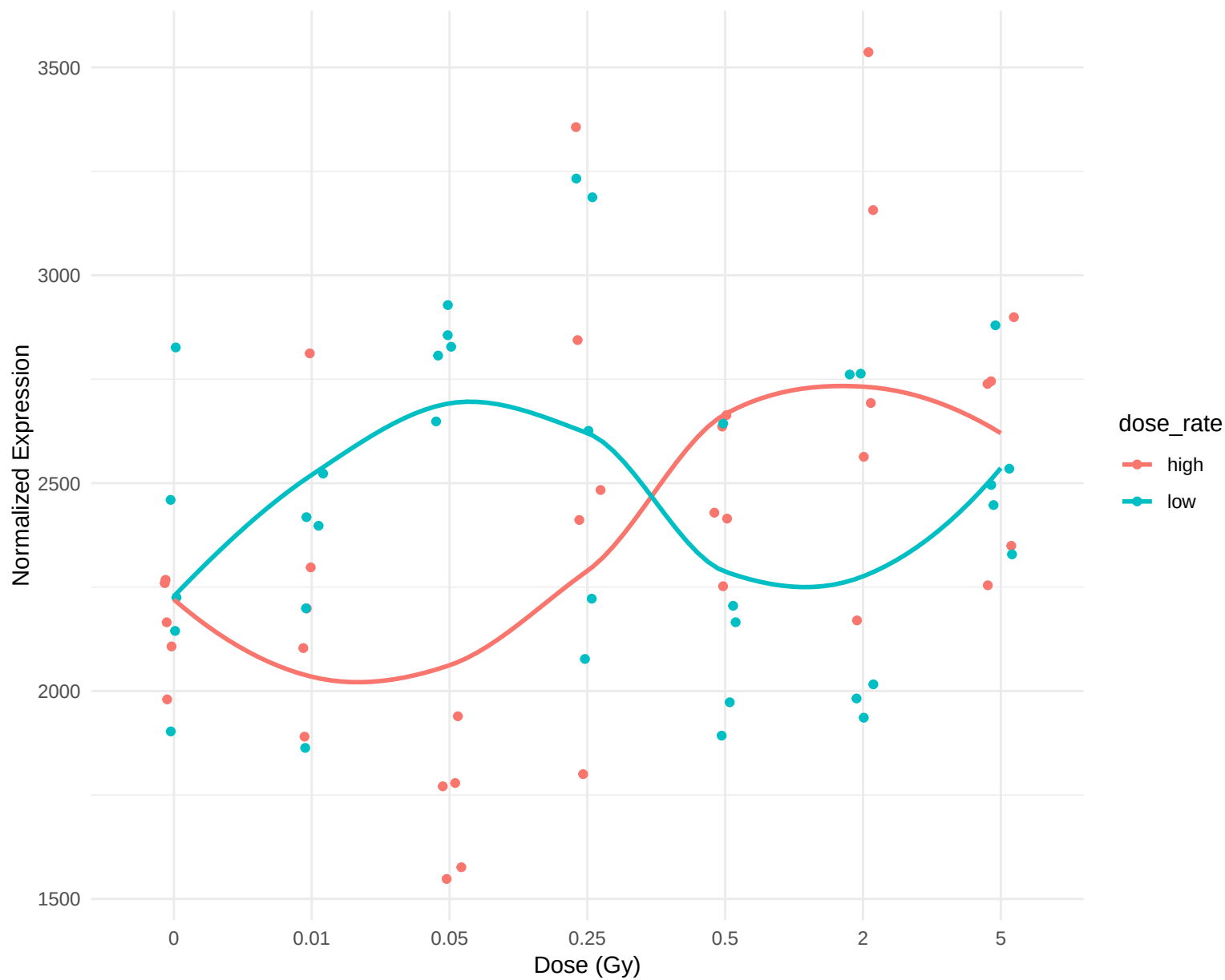
Rate-Dependent Response for ENSG00000221978
