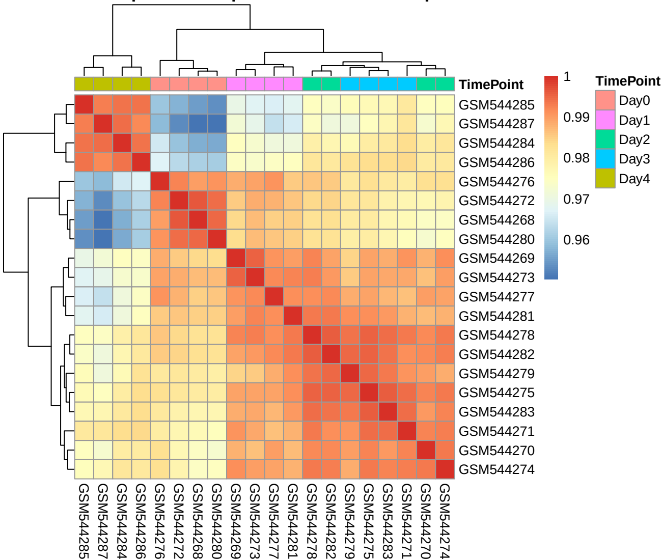
Sample-to-Sample Correlation Heatmap
