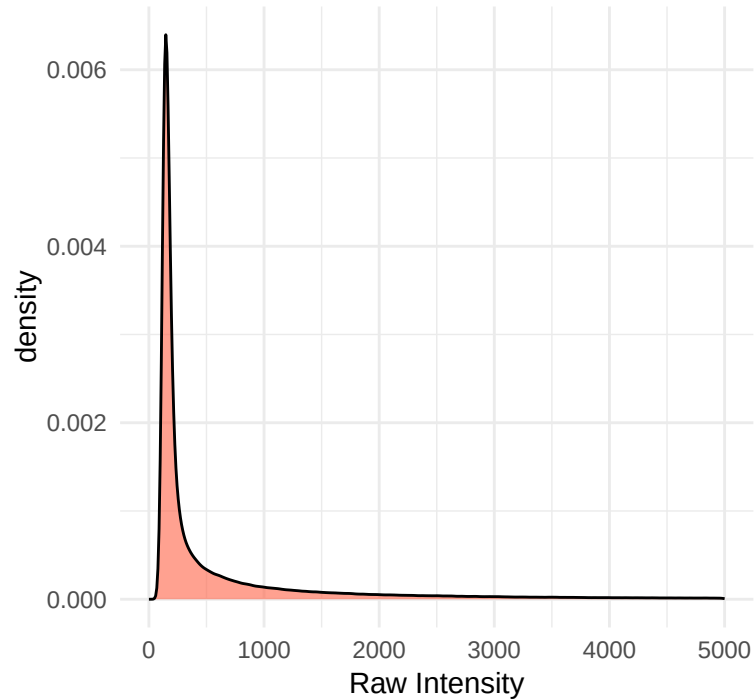
Before Log2 Transform
