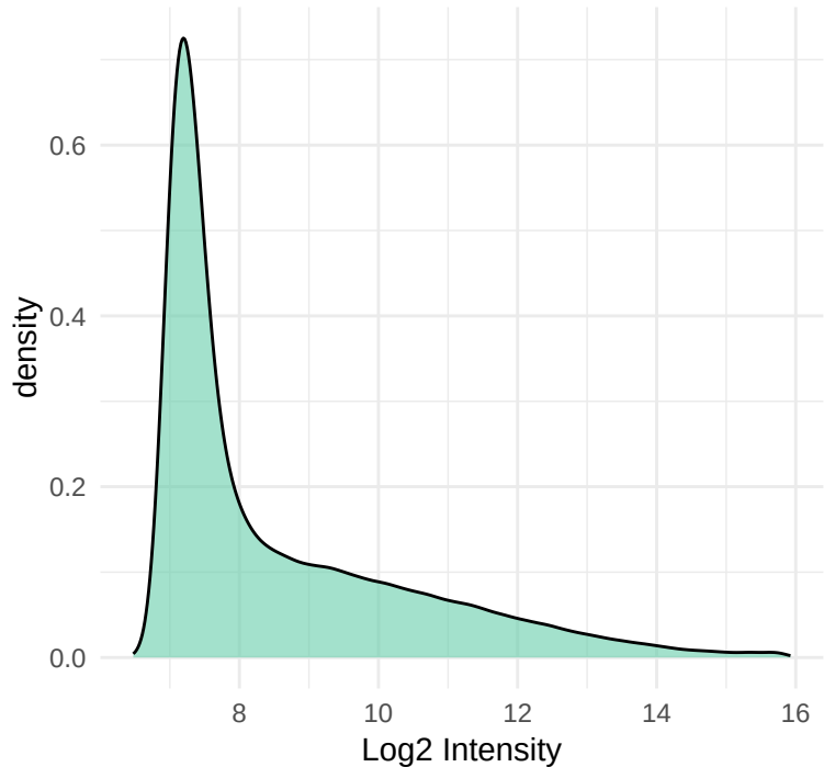
After Log2 Transform
