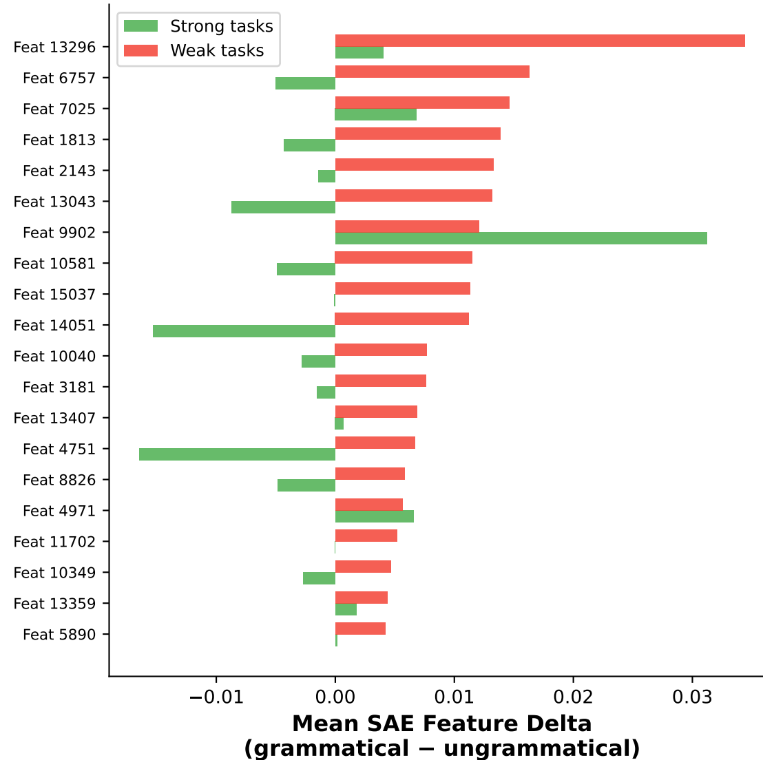
Top 20 Features: Weak Tasks (ranked by weak gram-ungram delta)
