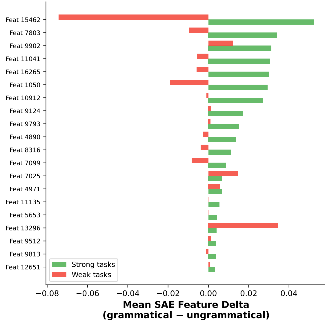
Top 20 Features: Strong Tasks (ranked by strong gram-ungram delta)
