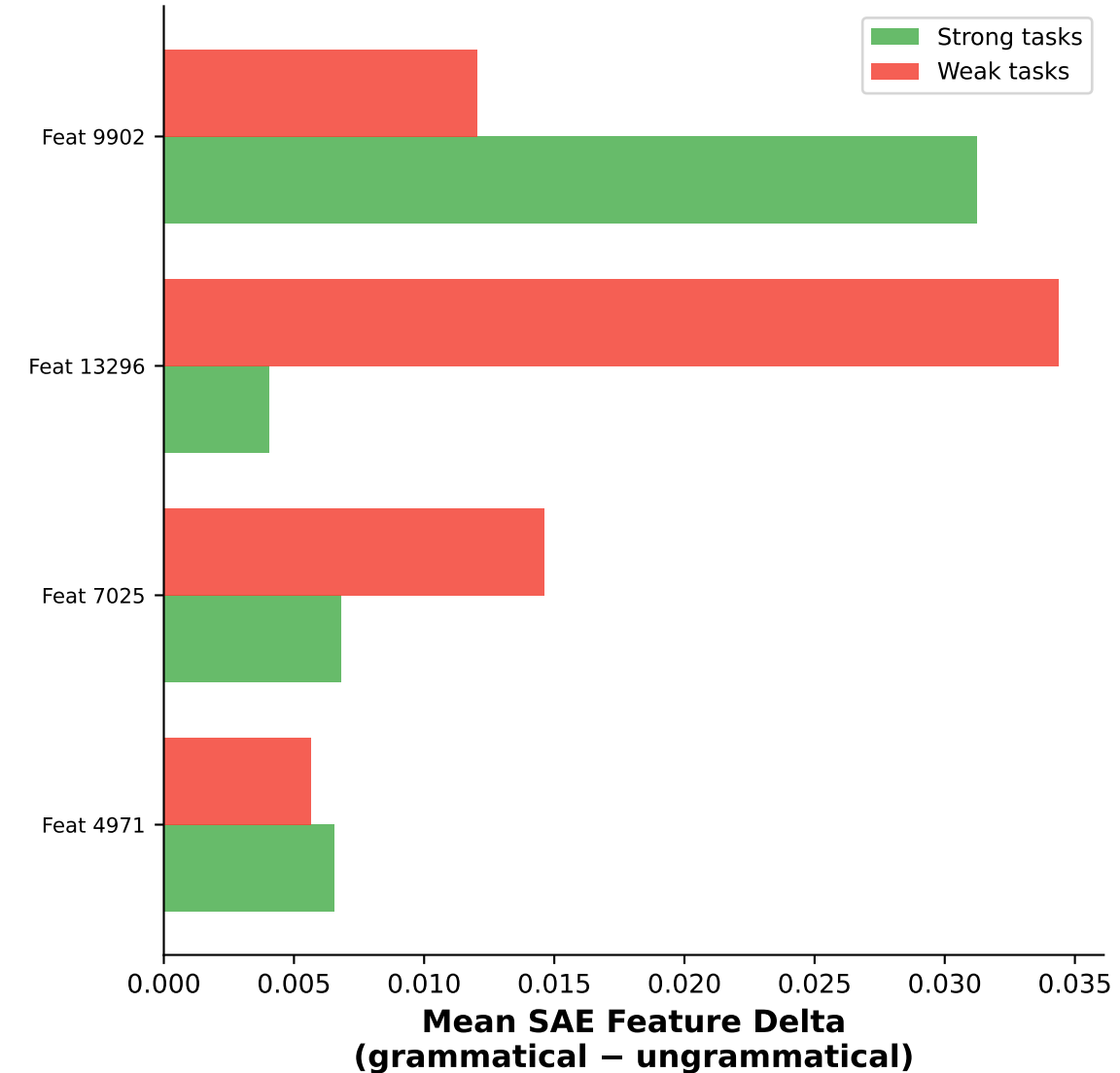
Shared Features (in both top-20) (4 found)
