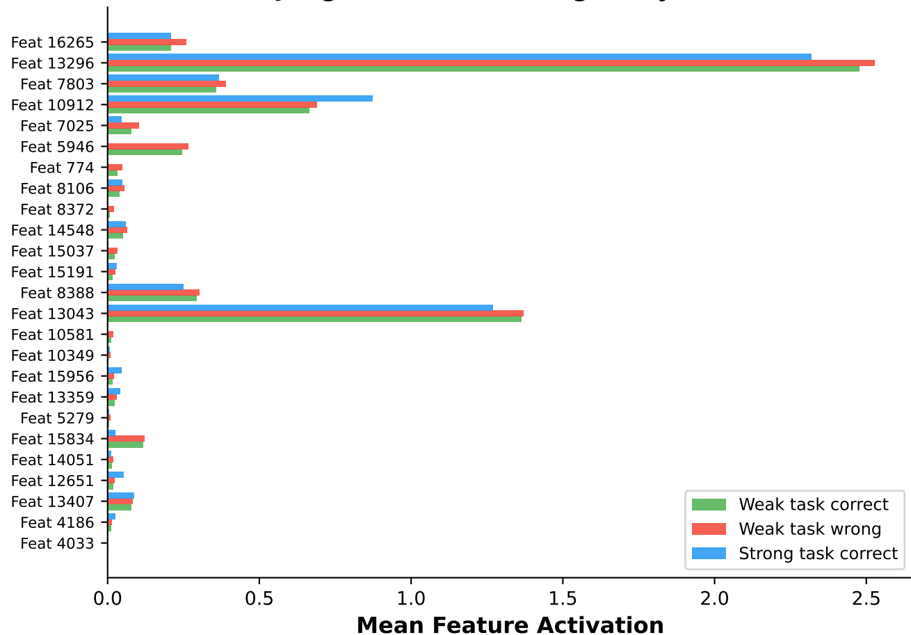
Features Active on Incorrect Judgments (Misleading) · Layer 12
