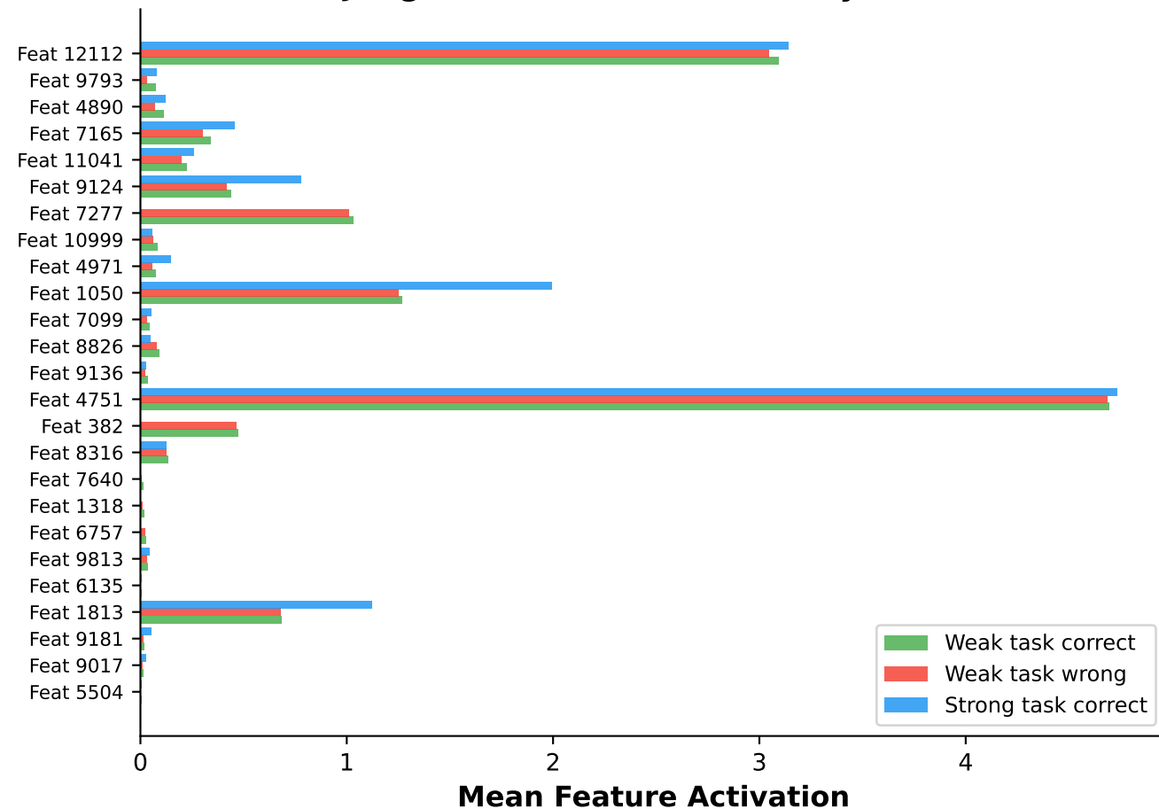
Features Predicting Correct Judgment on Weak Tasks (Layer 12)
