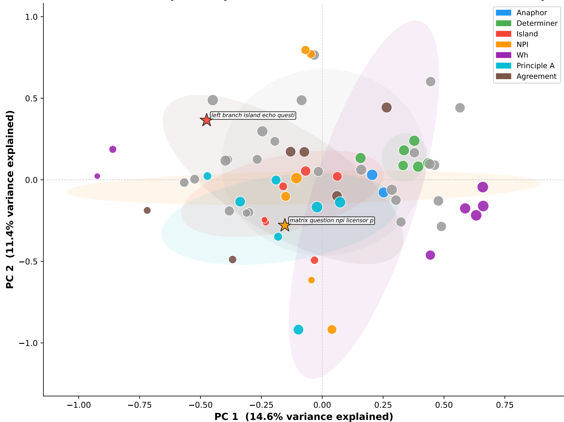
Geometry of Task Grammaticality Signals in SAE Space GPT-2 Medium (BabyLM) · Layer 12 (unit-normalised delta vectors · size \propto accuracy)
