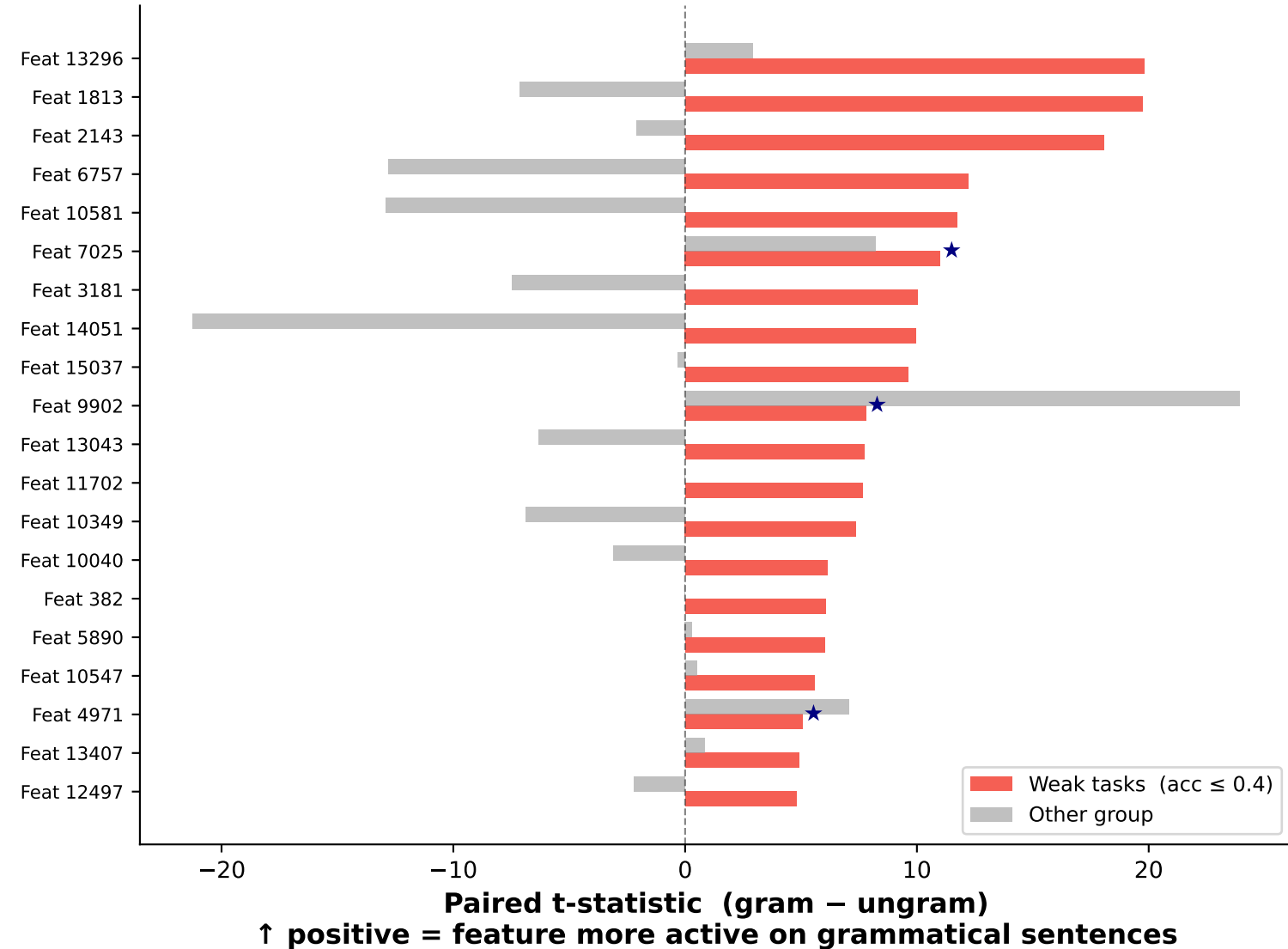
Top 20 by t-stat Weak tasks (acc ≤ 0.4)
