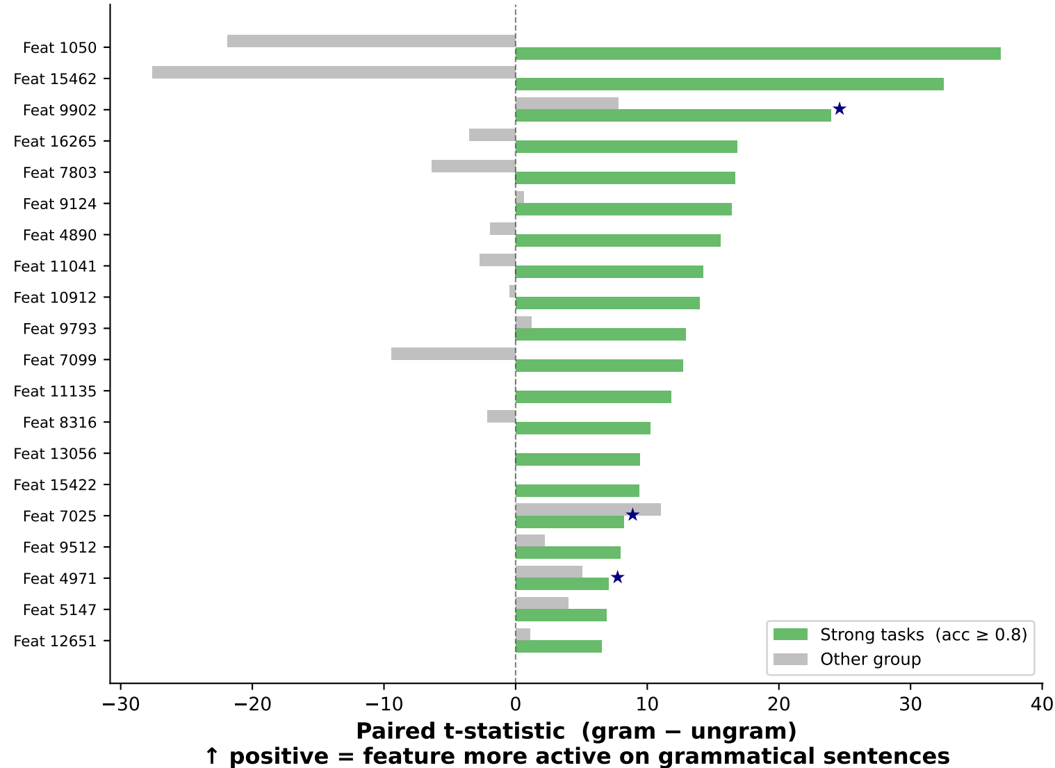
Top 20 by t-stat Strong tasks (acc ≥ 0.8)
