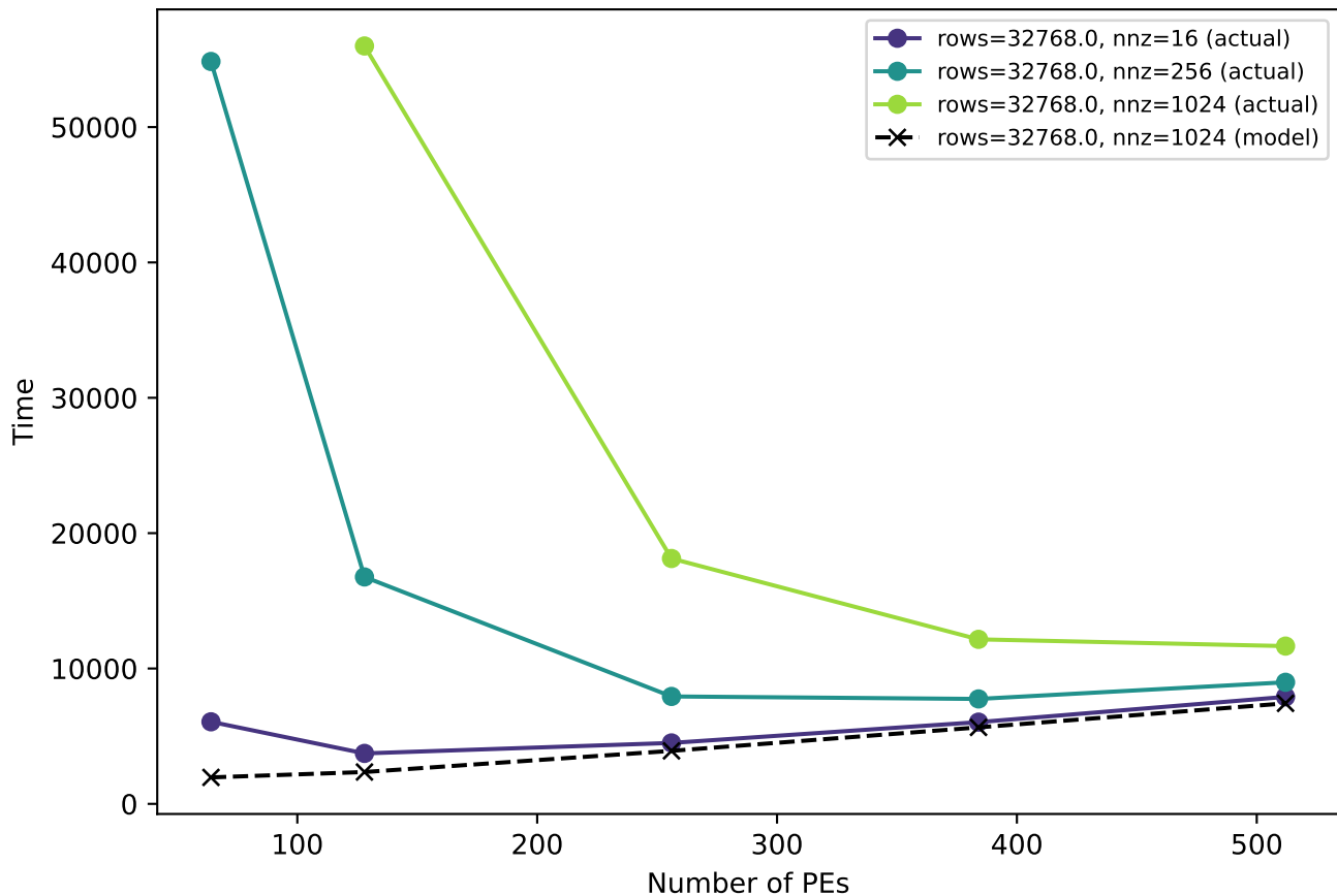
Comm Model vs Actual Runtime for Representative Cases
