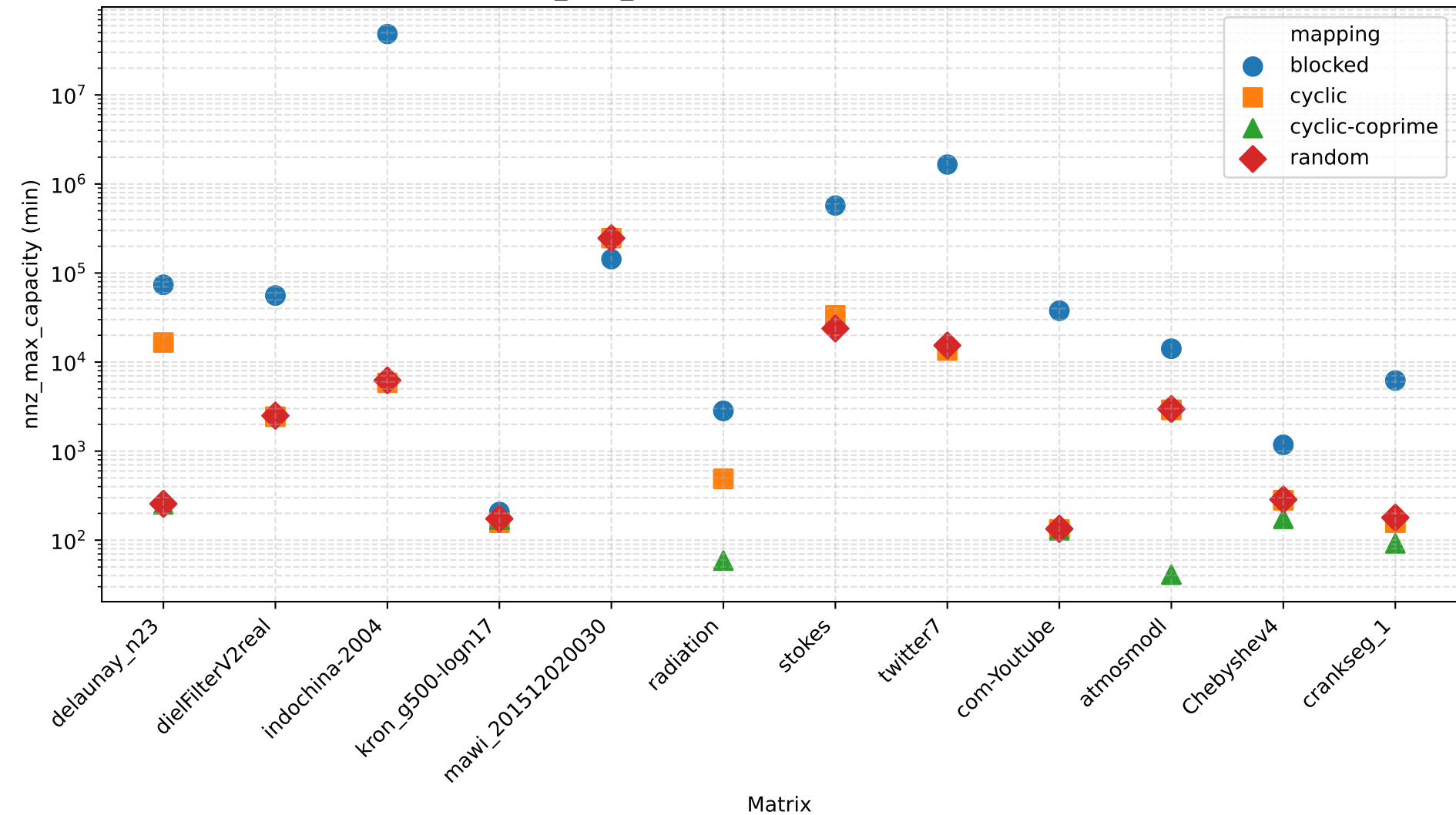
Min nnz_max_capacity per matrix, by mapping type
