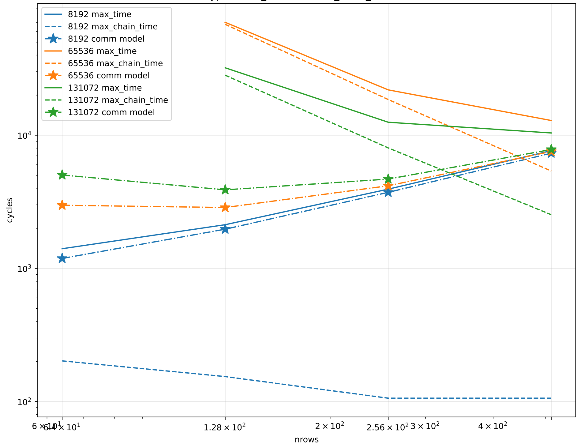
rand-4types: max_time and max_chain_time vs nrows
