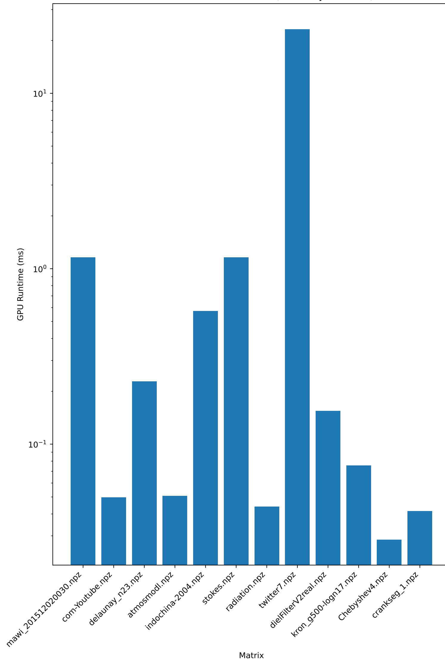
GPU Runtimes for Each Matrix (sorted by nnz/rows)
