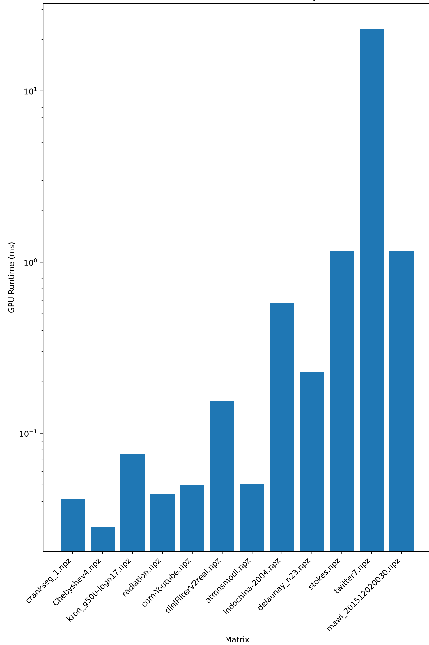
GPU Runtimes for Each Matrix (sorted by rows)
