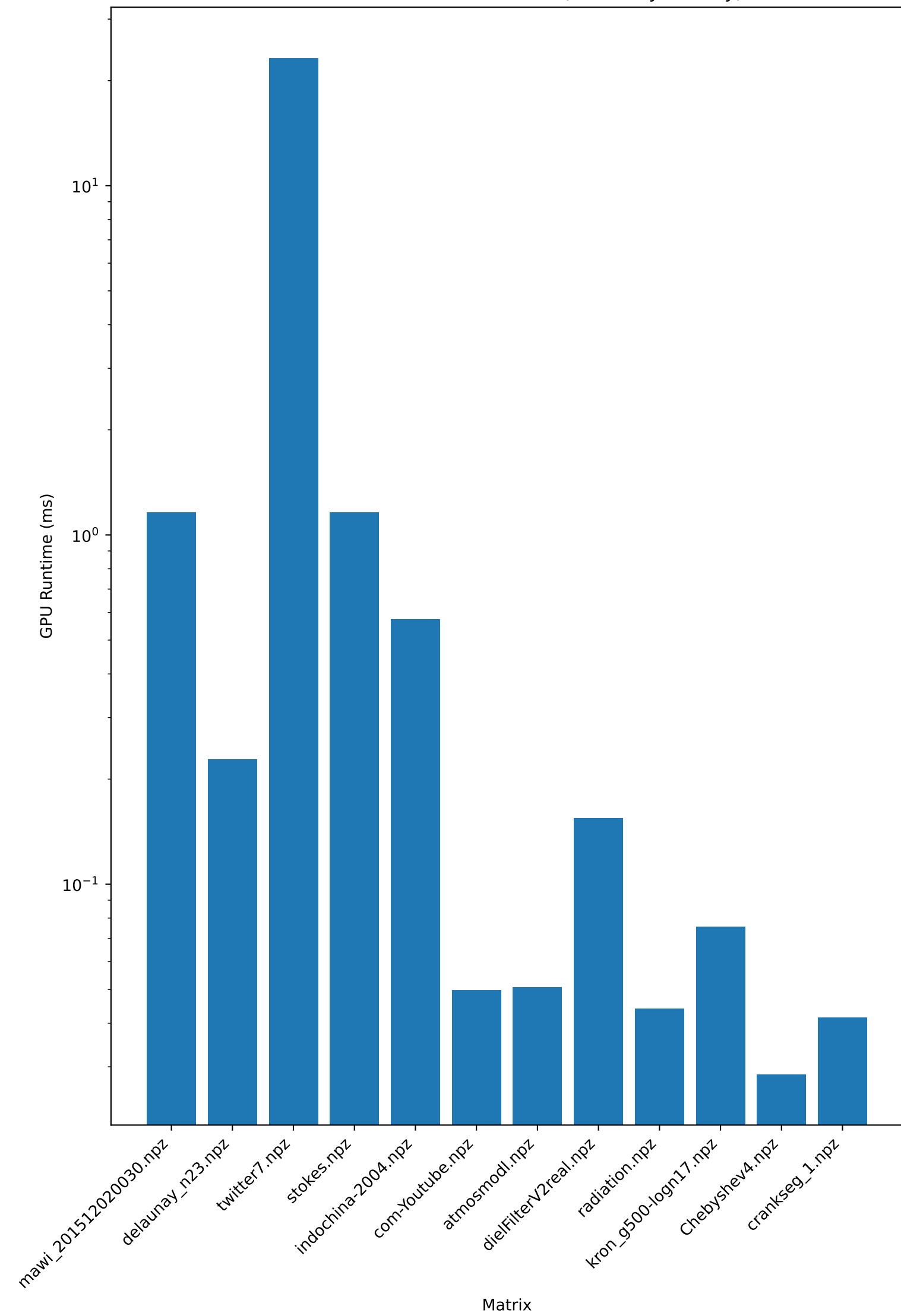
GPU Runtimes for Each Matrix (sorted by density)
