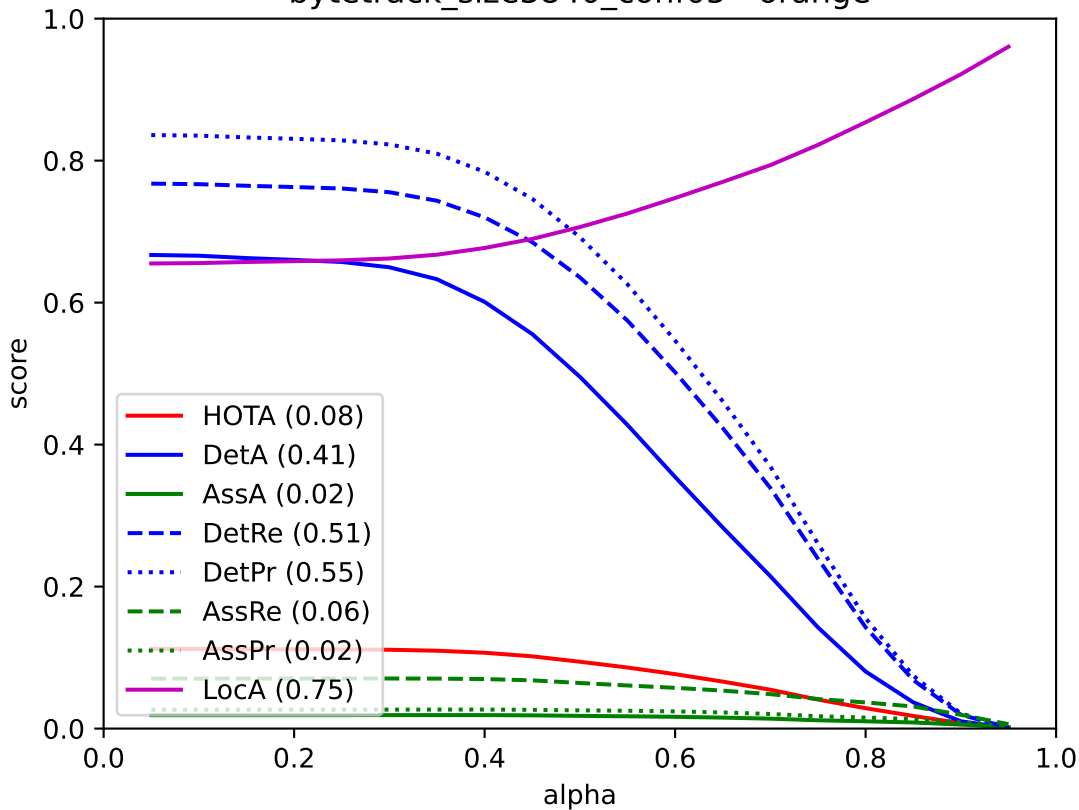
bytetrack_size3840_conf05 - orange
