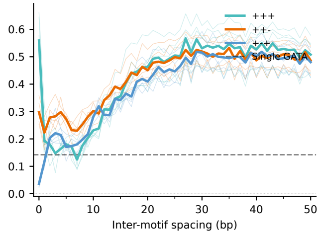
DNase
