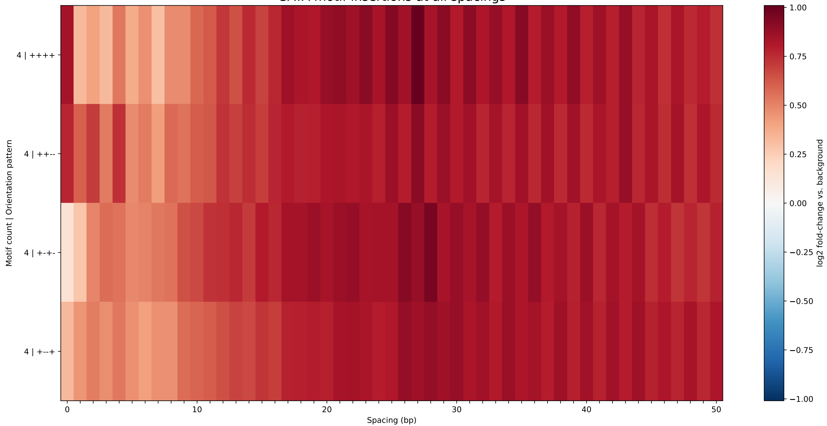
GATA motif insertions at all spacings
