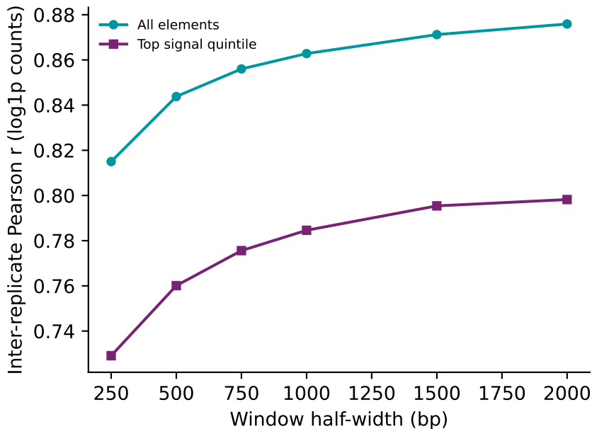
Achievable ceiling rises with window
