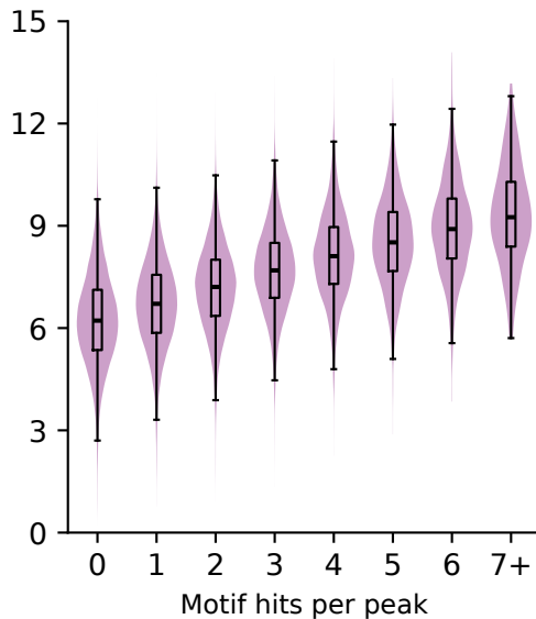
Predicted log counts
