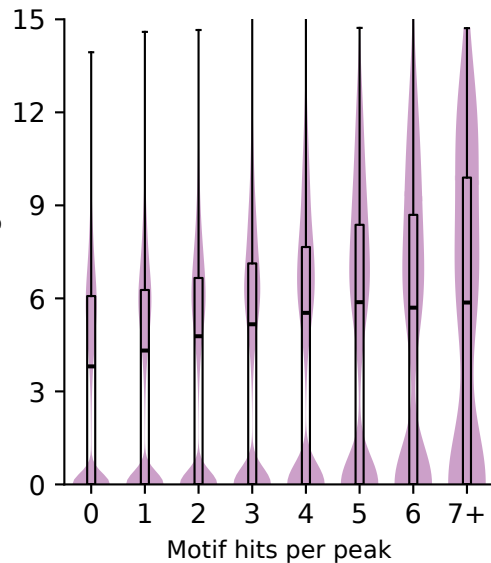
Observed log counts
