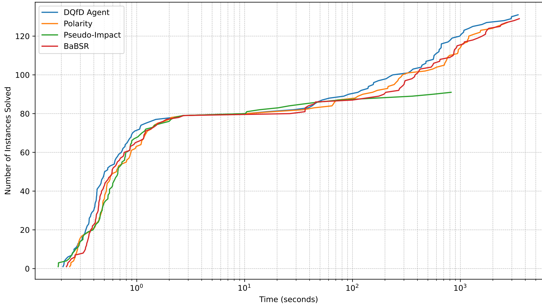
Performance (ACAS-Xu)
