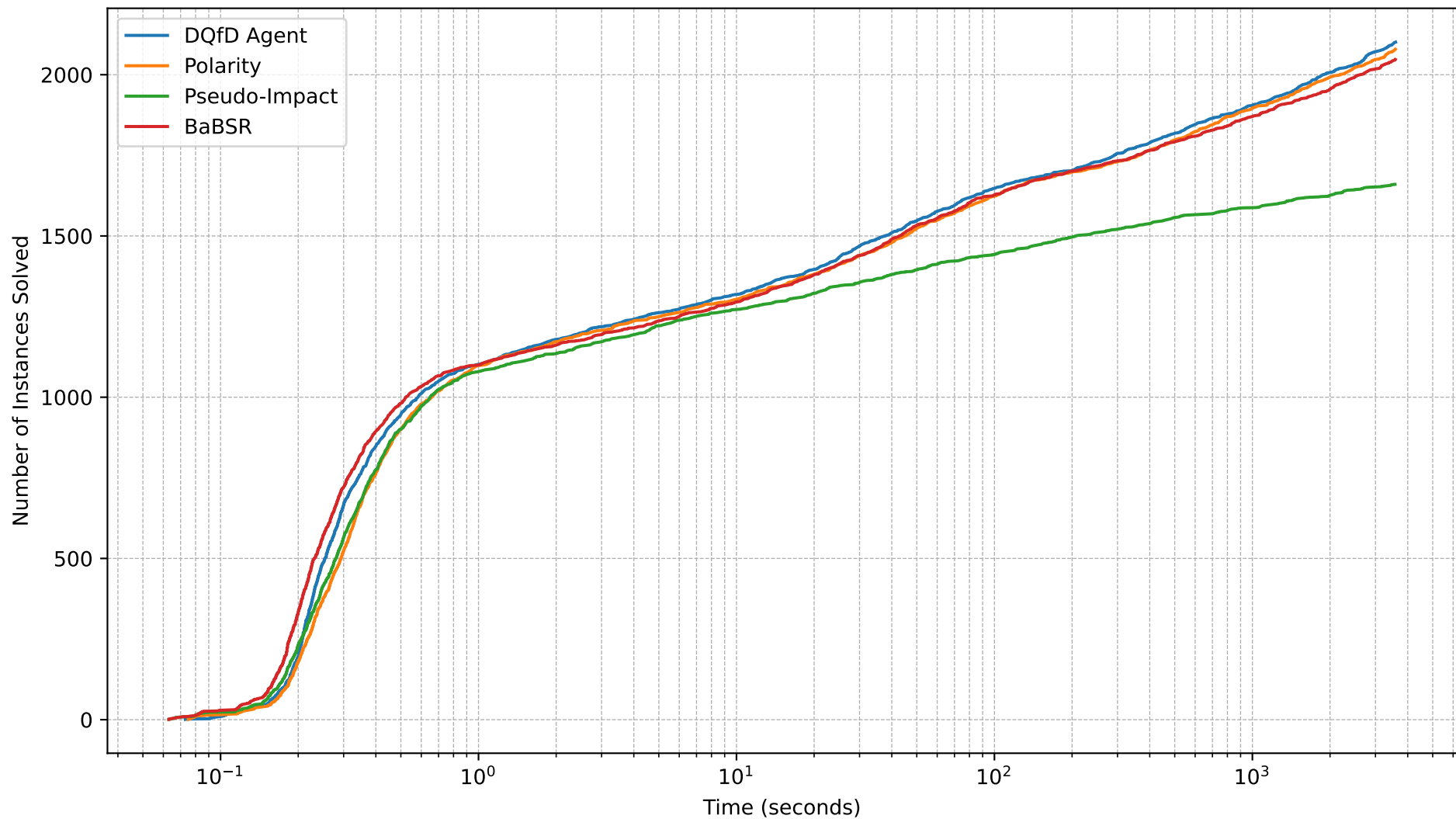
Performance (ACAS-Xu Robustness)
