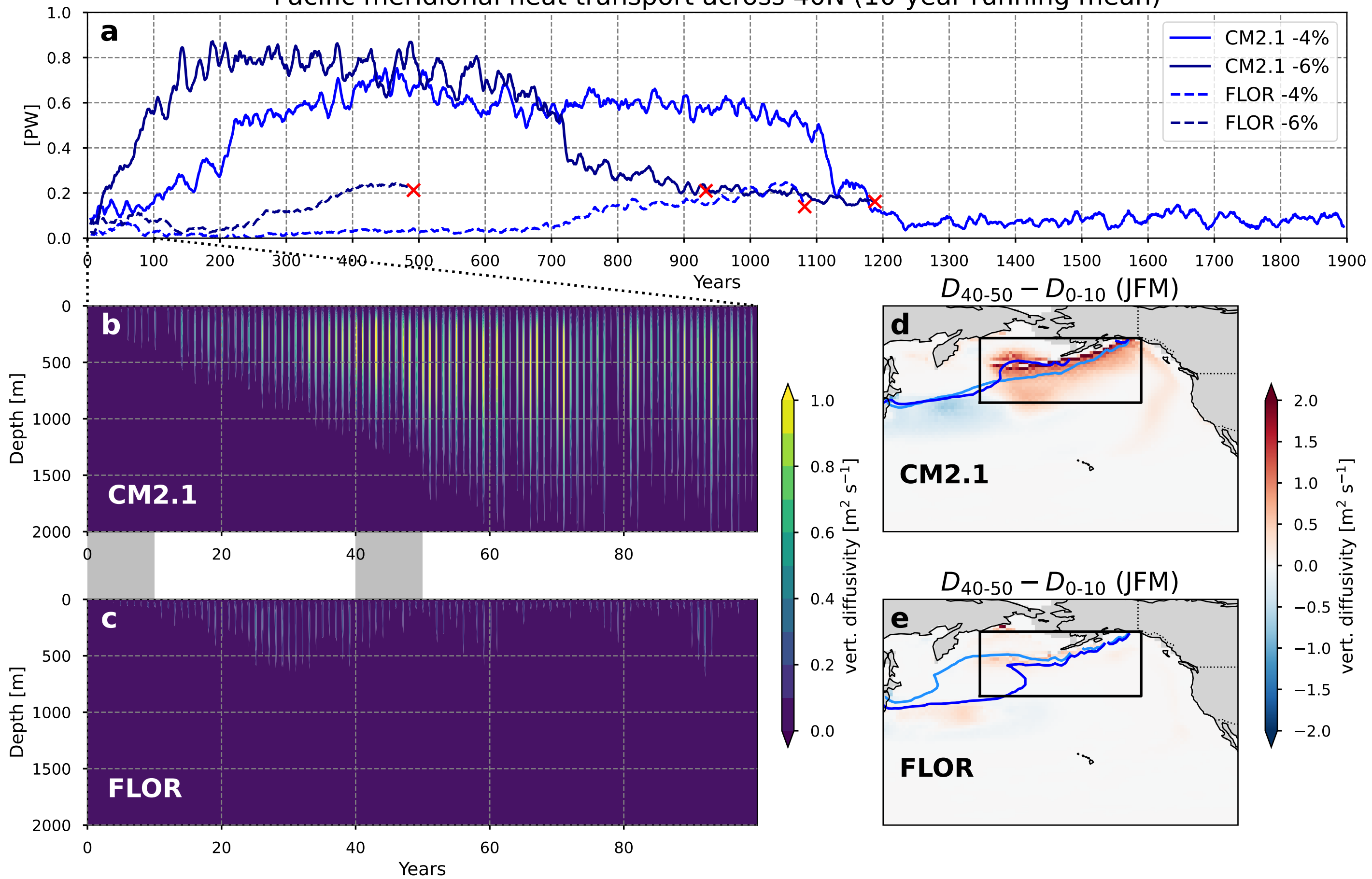
Pacific meridional heat transport across 40N (10-year running mean)
