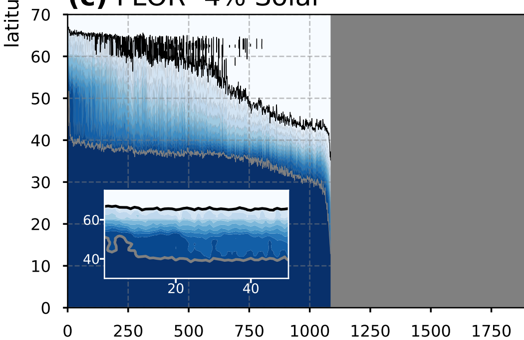
(c) FLOR -4% Solar
