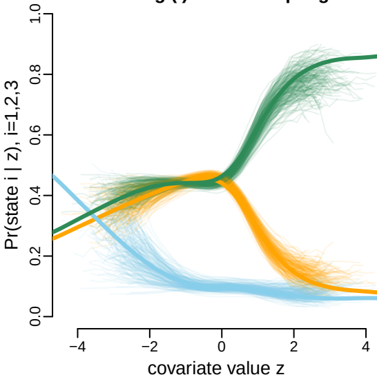
Setting (I): BB resampling
