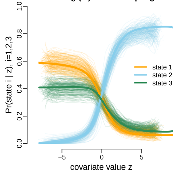
Setting (III): BB resampling
