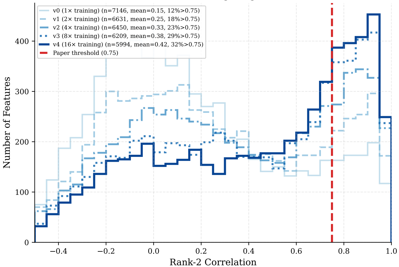
Rank-2 Correlation: Training Progression (v0 \rightarrow v4)
