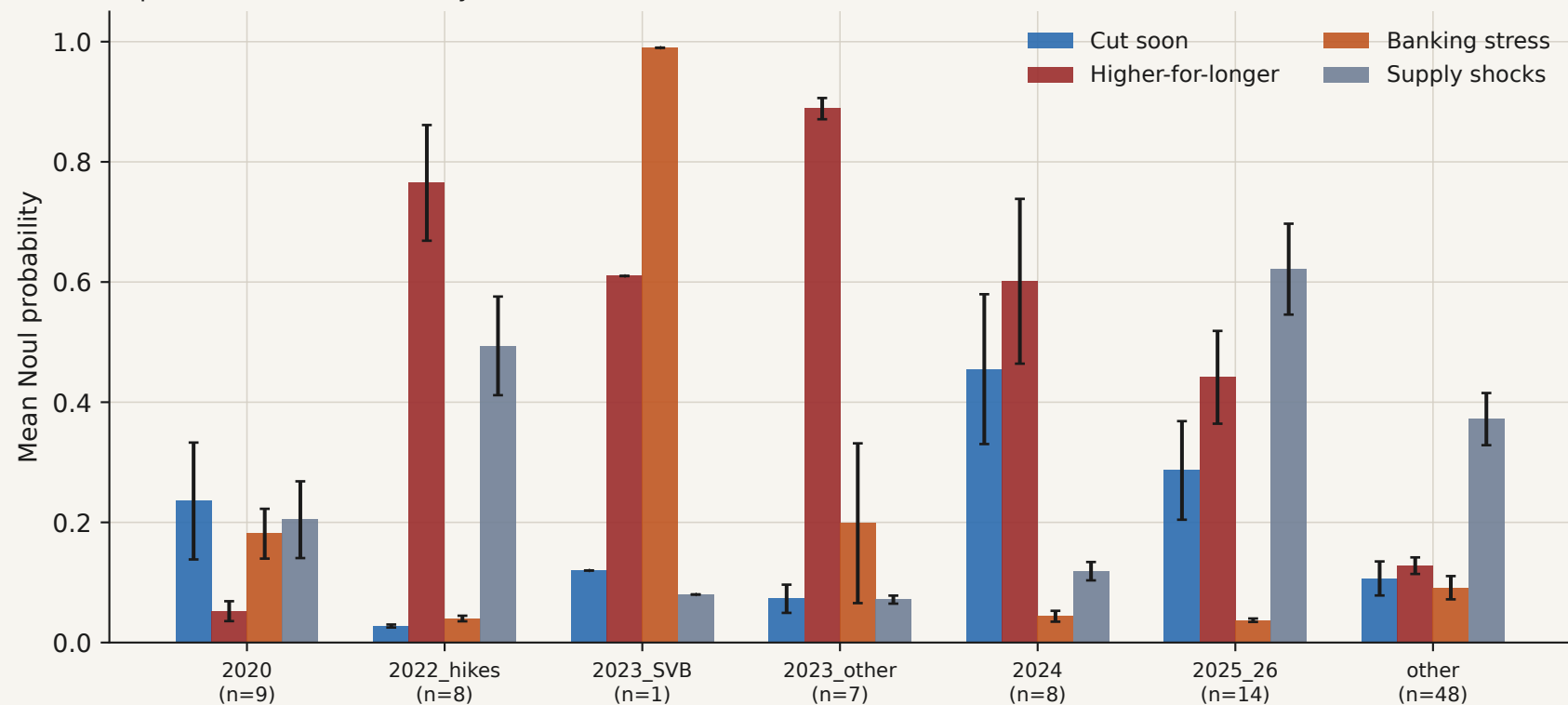
Exp. 4 — Multi-label Nouns by era (mean \pm STE)
