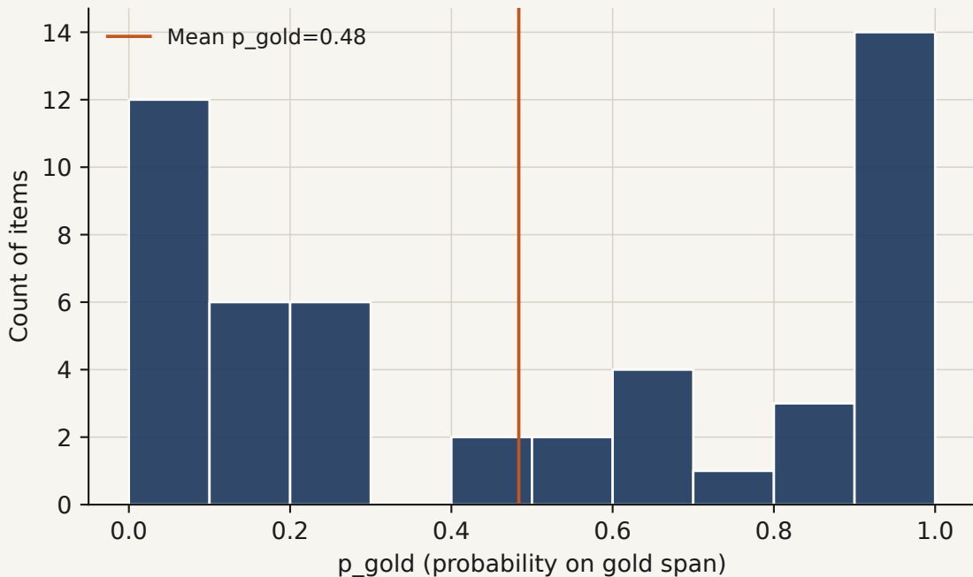
Exp. 6 — Span Choice p_{\text{gold}} distribution Inversion=0.48 (STE 0.07, n=50 )
