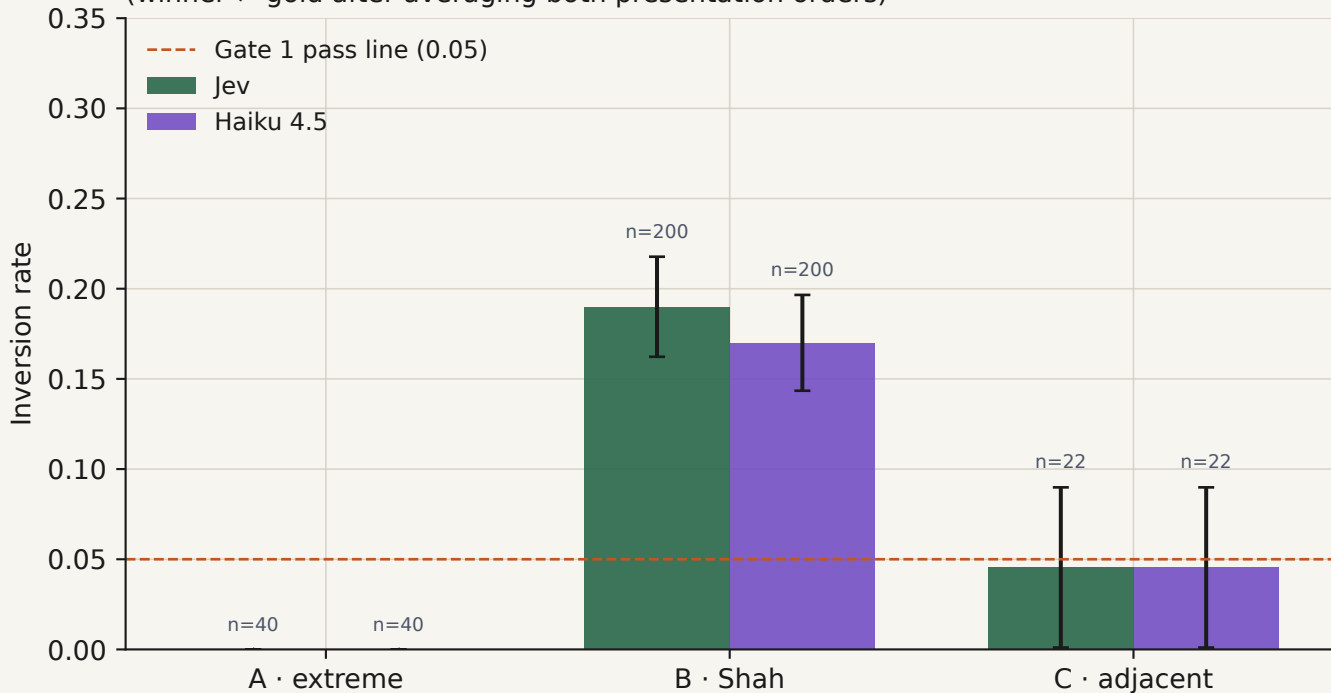
Gates 1-2 — Inversion rate \pm binomial STE by stratum (winner \neq gold after averaging both presentation orders)
