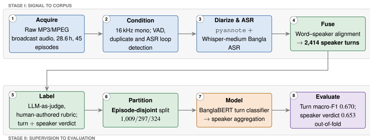
Figure 2. Technical pipeline followed in the course project. Splitting is grouped by episode, never by row, so that turns from one panel cannot appear on both sides of the split; the deduplicated episode is removed before partitioning. All 45 episodes carry trusted pyannote diarization in this build.
