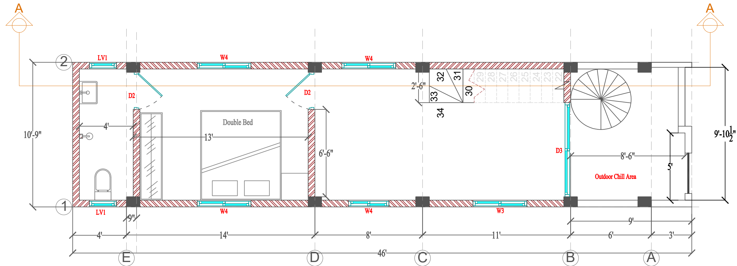
ROOF FLOOR PLAN
