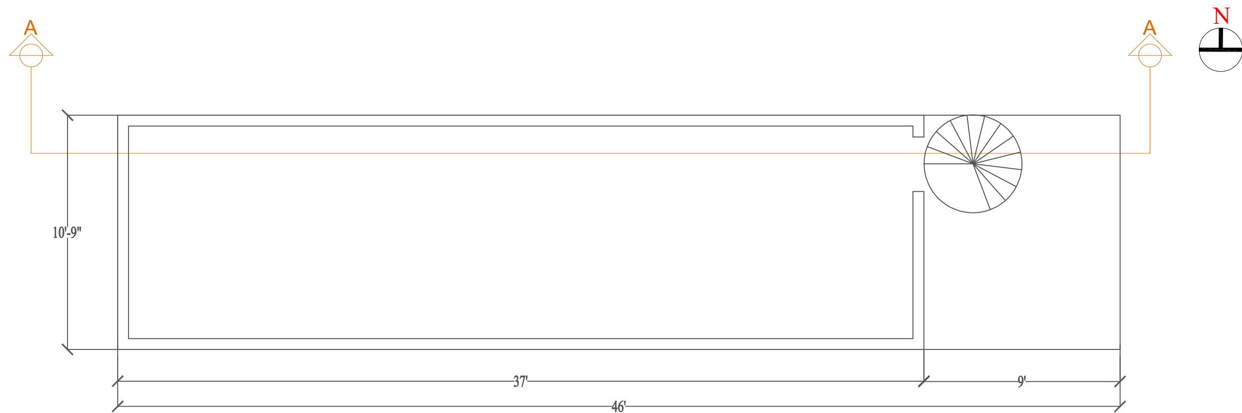
ROOF TOP PLAN
