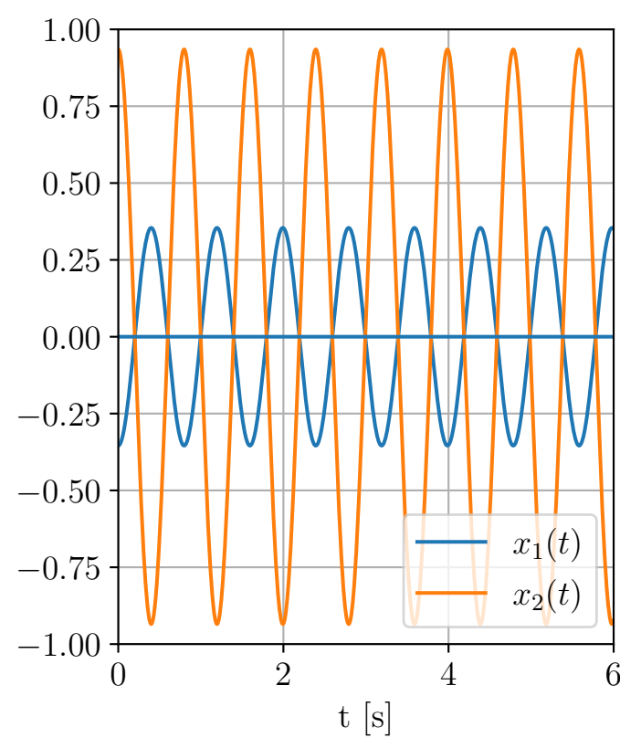
(c) Resposa en mode 2 a \omega_2 = 7.88 rad/s.
