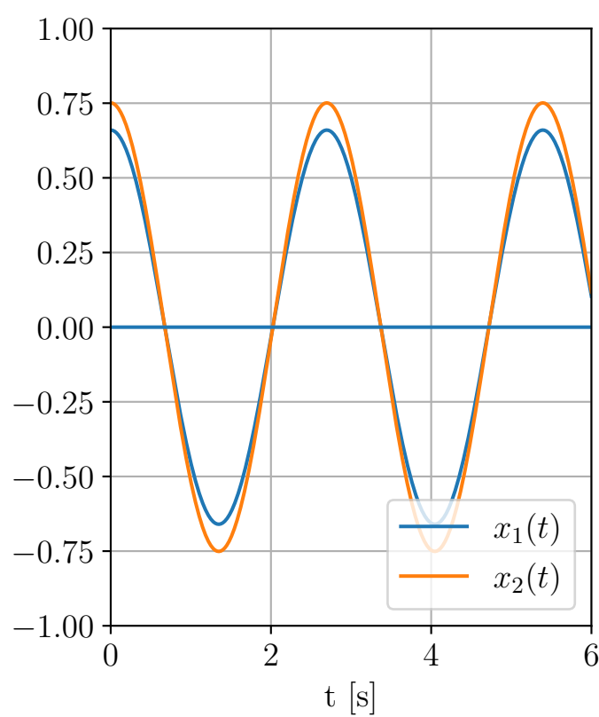
(b) Resposa en mode 1 a \omega_1 = 2.33 rad/s.
