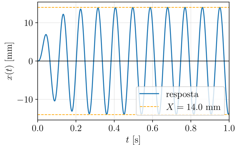
(a) Resposta a F(t) = 120 \sin(22\pi \cdot t) N
