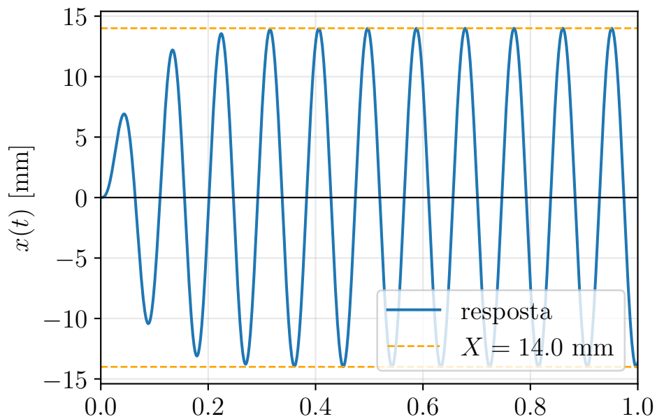
(a) Resposta a F(t) \stackrel{t[s]}{=} 120 \sin(22\pi \cdot t) N
