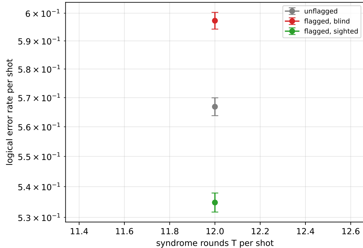
[[46, 2, 9]], p = 0.003 , 100,000 shots/arm
