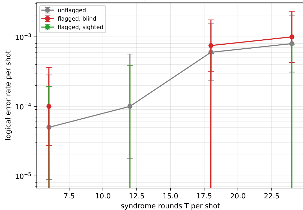
[[144, 12, 12]], p = 0.001 , 20,000 shots/arm
