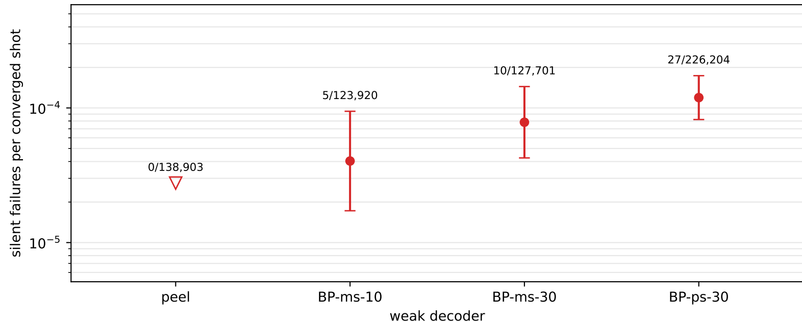
How often is each weak decoder confidently wrong? ( \nabla = none seen: 95% upper bound)
