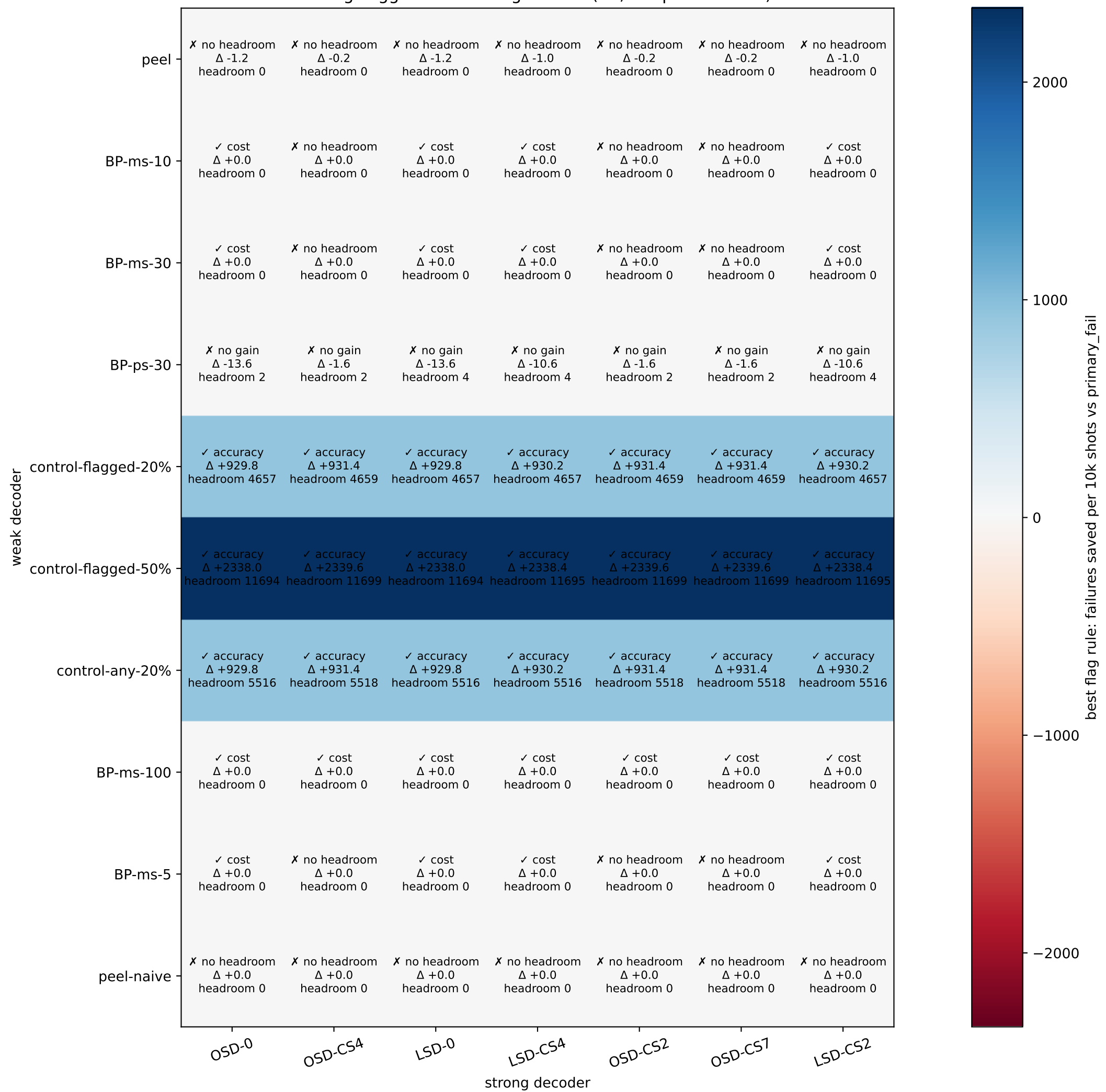
Is flag-triggered switching viable? (50,000 paired shots)
