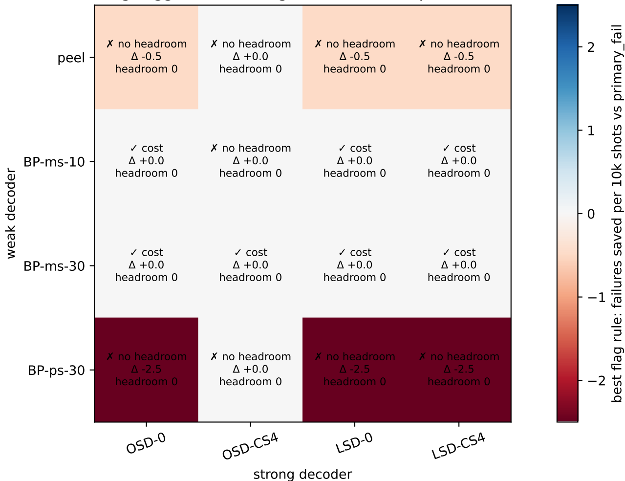
Is flag-triggered switching viable? (20,000 paired shots)
