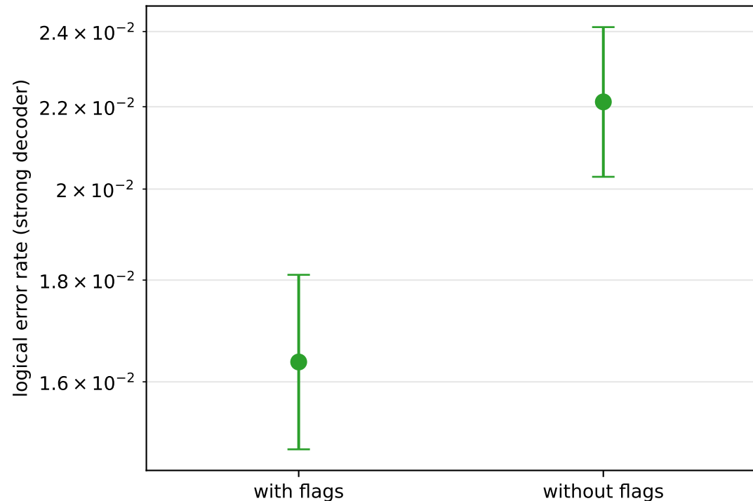
V3 — flags improve accuracy
