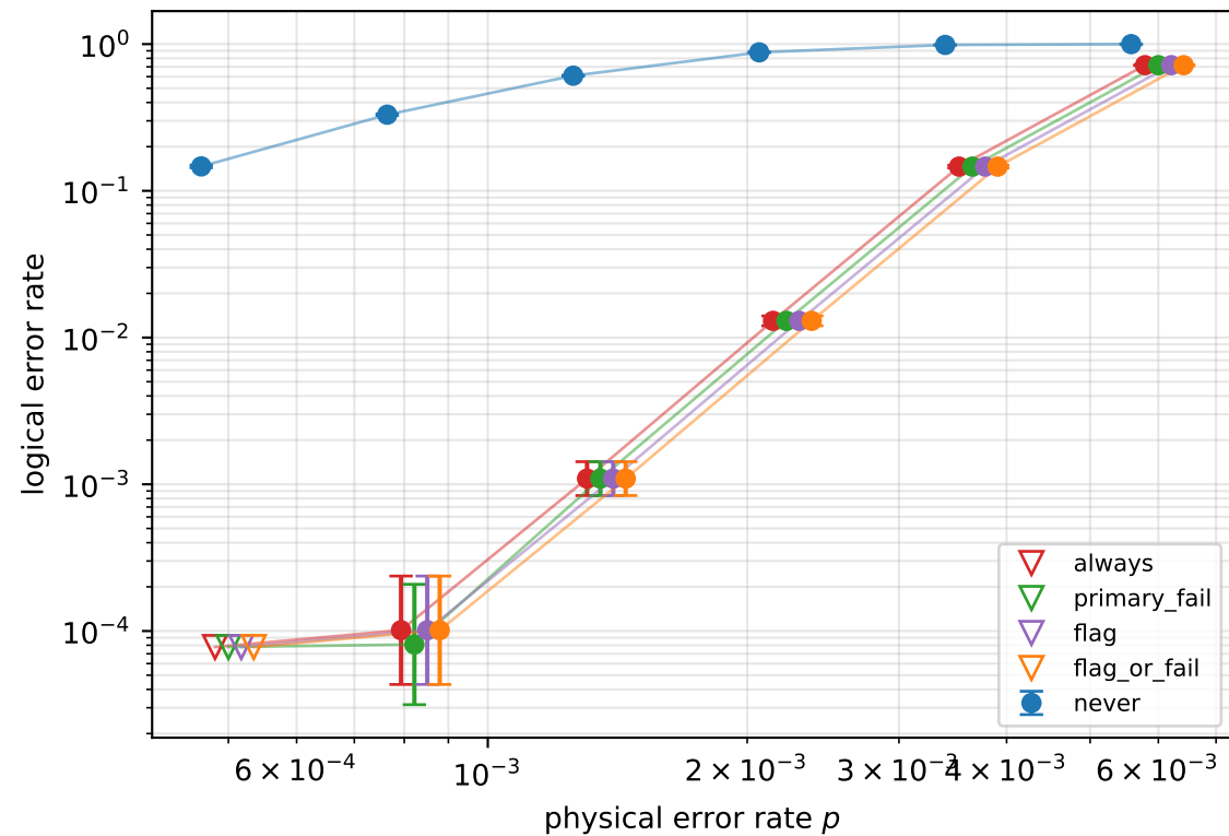
(a) accuracy ( \nabla = 95% upper bound, no failures) points offset sideways slightly so overlaps stay visible
