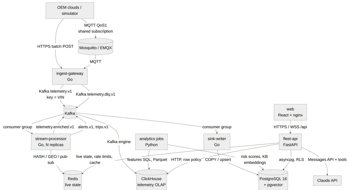
Figure 4. Containers (C4 level 2), with the protocol on each arrow.
