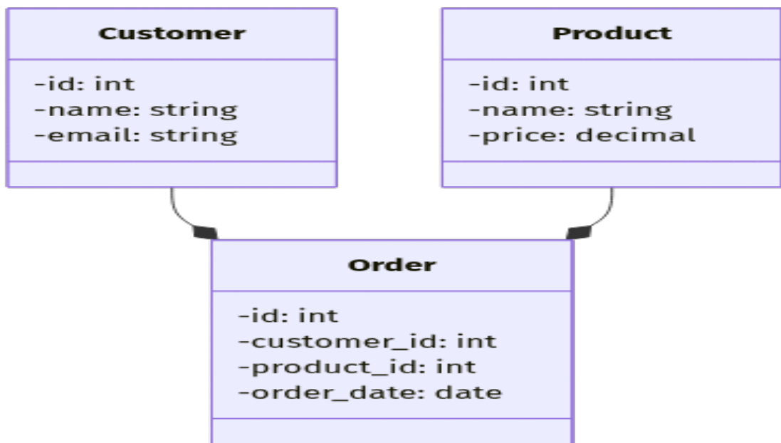
Figure 13.1: Industrial online-library/online-library/diagram 2.3.jpg Schematic
