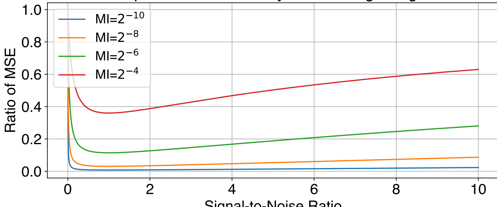
MSE Improvement in Privacy-Aware Ridge Regression
