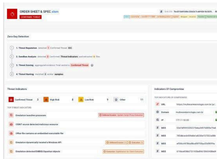
Figure 11 – FileScan.io Overview – ORDER SHEET & SPEC.xlsm – Confirmed Threat, 3 Malicious Indicators, Tags: xlm/exploit/dropper/evasive/macros
