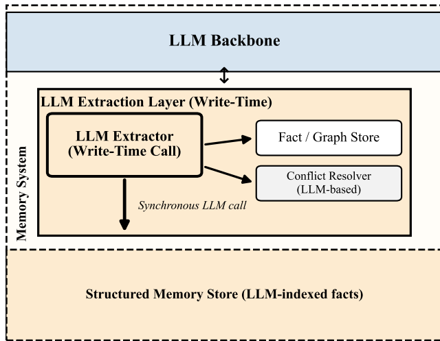
(b) Coupled (e.g., Mem0, LangMem, Graphiti)
