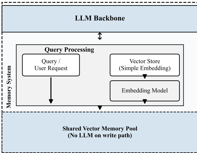
(a) Decoupled (e.g., Naive RAG)
