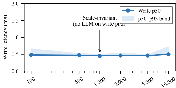
(a) Write Latency vs. Scale
