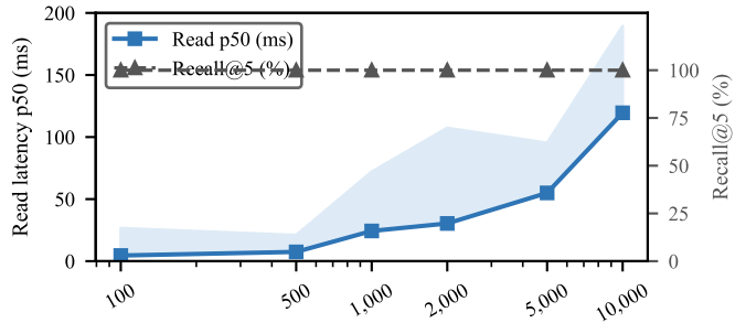
(b) Read Latency & Recall vs. Scale
