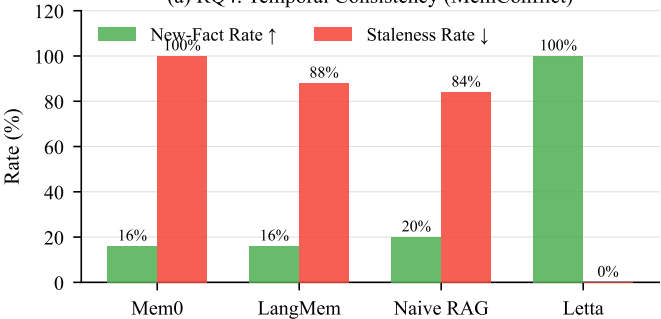
(a) RQ4: Temporal Consistency (MemConflict)
