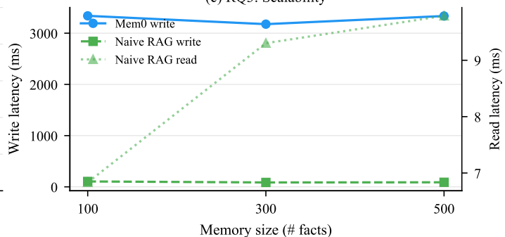
(c) RQ3: Scalability
