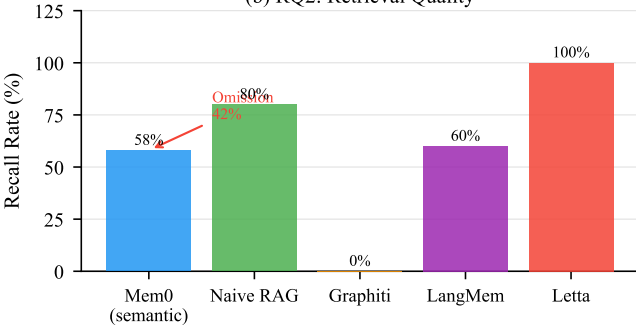
(b) RQ2: Retrieval Quality
