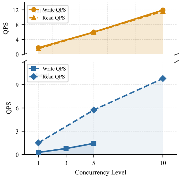
(b) Throughput (QPS) vs. Concurrency
