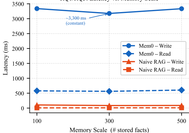
RQ1/RQ3: Latency vs. Memory Scale
