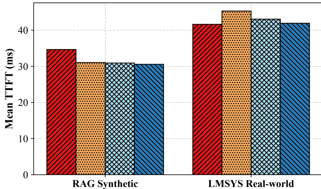
(b) Time to First Token
