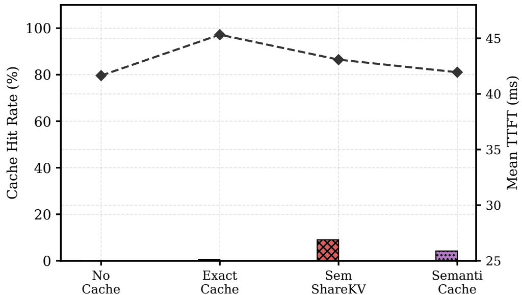
(b) LMSYS Real-world (n=500)
