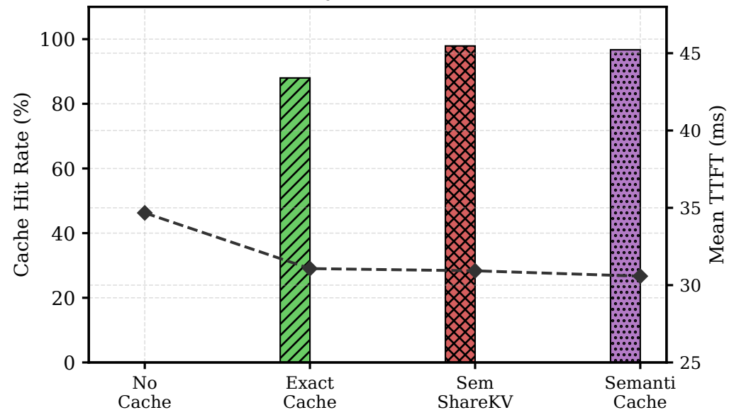
(a) RAG Synthetic (n=1,000)
