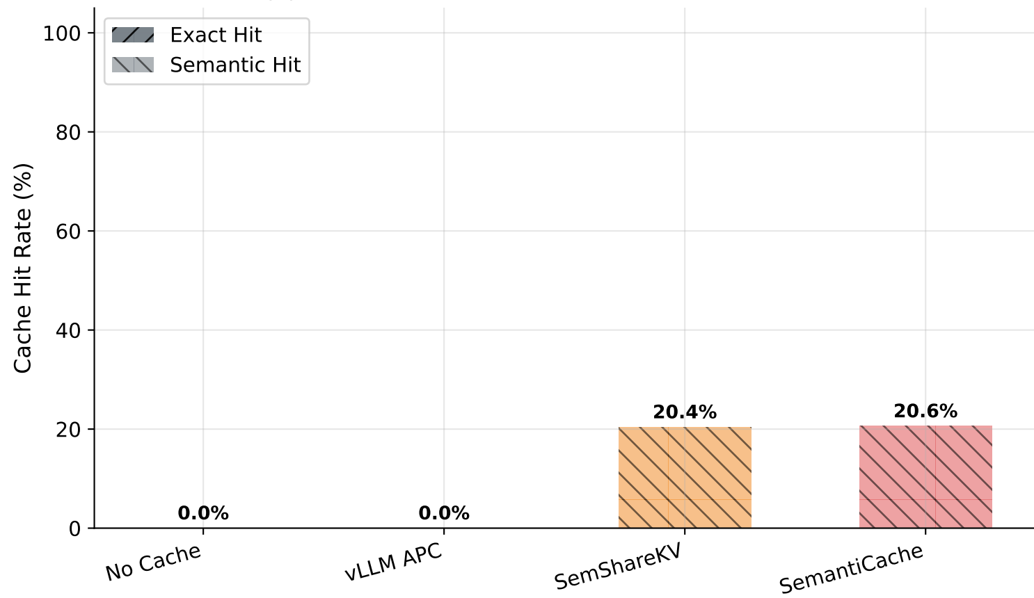
(a) Cache Hit Rate — SemantiCache vs. Baselines
